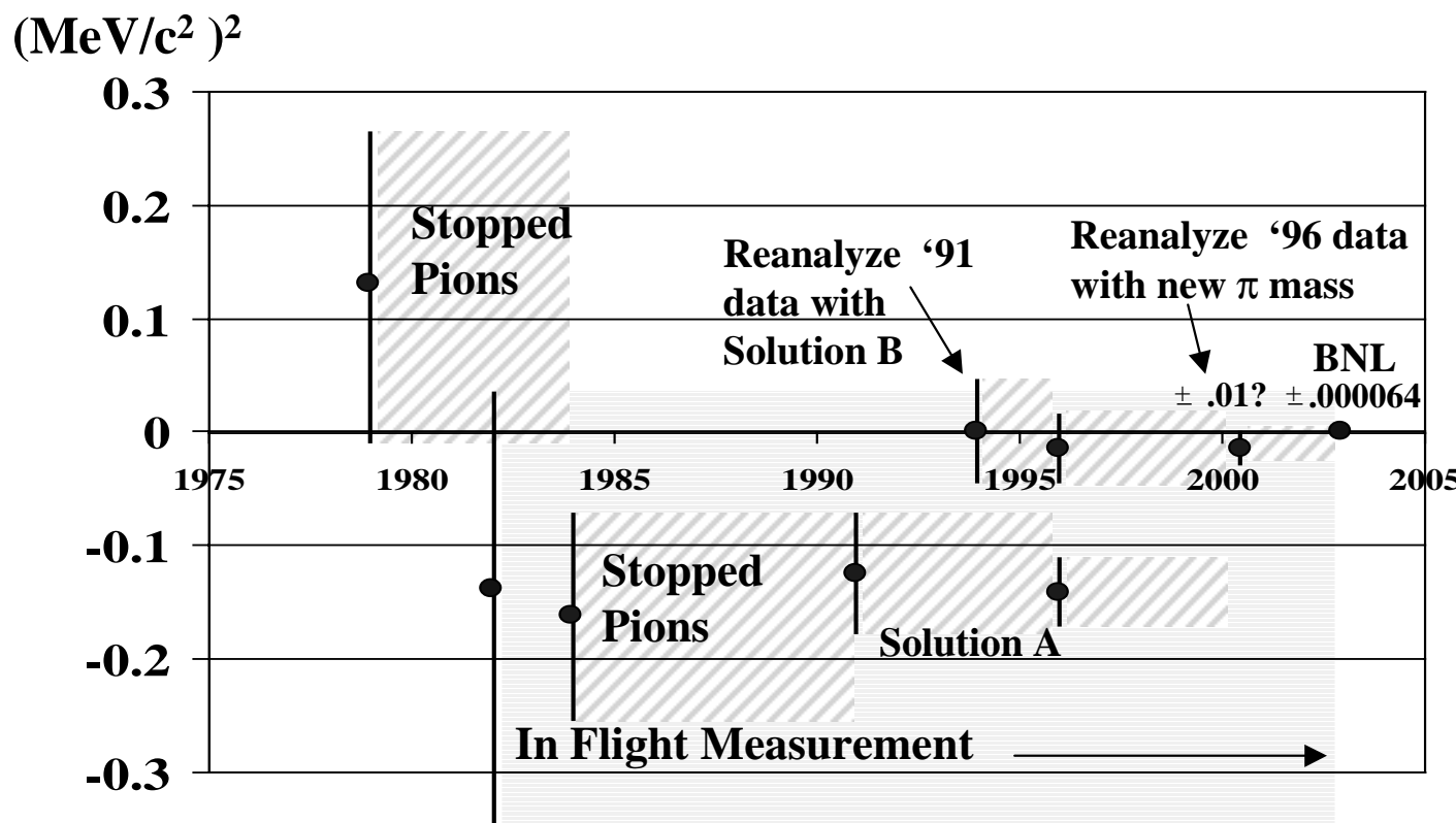
Measurements of m^2(\nu_\mu) by year
