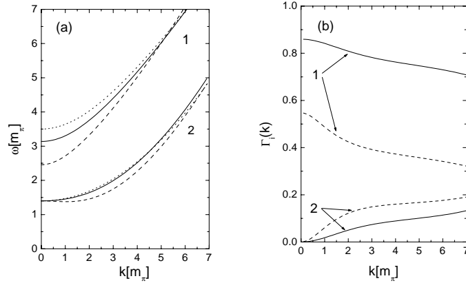
Fig. 1. Spectrum of K^- (\bar{K}^0) mesons (left panel (a)) and occupation factors \Gamma_i(k) (right panel (b)) in isotopically symmetrical nuclear matter calculated with the in-medium Green's function (4) at the breakup density \rho_b = 0.6\rho_0 (solid lines) and at a certain initial density \rho_m = 3\rho_0 (dashed lines). The kaon branch \omega_K(k) is labeled by 1, whereas the \Lambda branch \omega_\Lambda(k) is labeled by 2. The dotted lines depict the free kaons ( \omega = \sqrt{m_K^2 + k^2} ) and the free \Lambda ( \omega = \sqrt{m_\Lambda^2 + k^2} - m_N ). Kaon frequency and momentum are displayed in pionic units.
