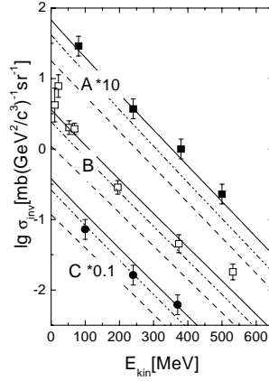
Fig. 3. The logarithm of the invariant differential cross section \omega_k \frac{d\sigma_{K^-}}{d^3k} \left[ \frac{mb}{GeV^2} \right] of K^- production as a function of the center-of-mass kinetic energy of kaons calculated via eq. (15) for ^{58}Ni + ^{58}Ni collisions at E_{lab} = 1.85 AGeV (curves A) and for ^{28}Si + ^{28}Si (B) and ^{21}Ne + ^{22}Ne (C) collisions at E_{lab} = 2.1 AGeV. Dashed curves are calculated with the free kaon spectrum, whereas dash-dotted curves employ the kaon polarization operator of ref. 7 , which includes only the s-wave KN interaction. Experimental data are from ref. 5 for Ni , 2,3 for Si and 4 for Ne .
