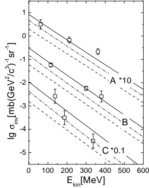
Fig. 4. The same as in Fig. 3, but for ^{28}\text{Si} + ^{28}\text{Si} collisions at collision energies E_{\text{lab}} = 1.65 AGeV (curves A), 1.4 AGeV (B) and 1.16 AGeV (C). The experimental data are from refs. 3,4 .
