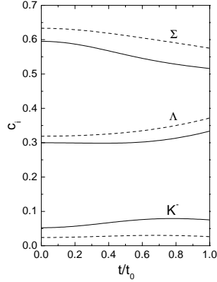
Fig. 2. Time evolution of the relative weights of the negatively strange particles c_K = c_{K^-} = c_{\bar{K}^0} , c_\Lambda and c_\Sigma for K^- ( \bar{K}^0 ), \Lambda and \Sigma , respectively, calculated with the in-medium kaon spectrum (solid lines) and the free kaon spectrum (dashed lines). Initial and final temperatures (densities) are equal to T_m = 133 MeV ( \rho_m = 3\rho_0 ) and T_b = 92 MeV ( \rho_b = 0.6\rho_0 ) corresponding (in accordance with refs. 13,18 ) to the beam energy E_{\text{lab}} = 2.1 AGeV.
