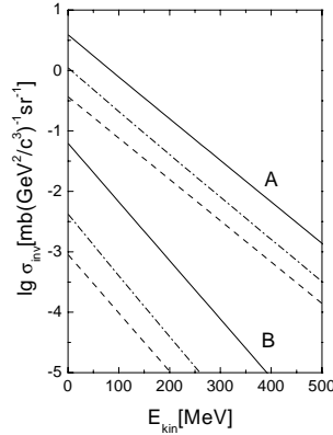
Fig. 5. The same as in Fig. 3, but for ^{197}\text{Au} + ^{197}\text{Au} reactions at E_{\text{lab}} = 1 AGeV (curves A) and at E_{\text{lab}} = 0.5 AGeV (B).
