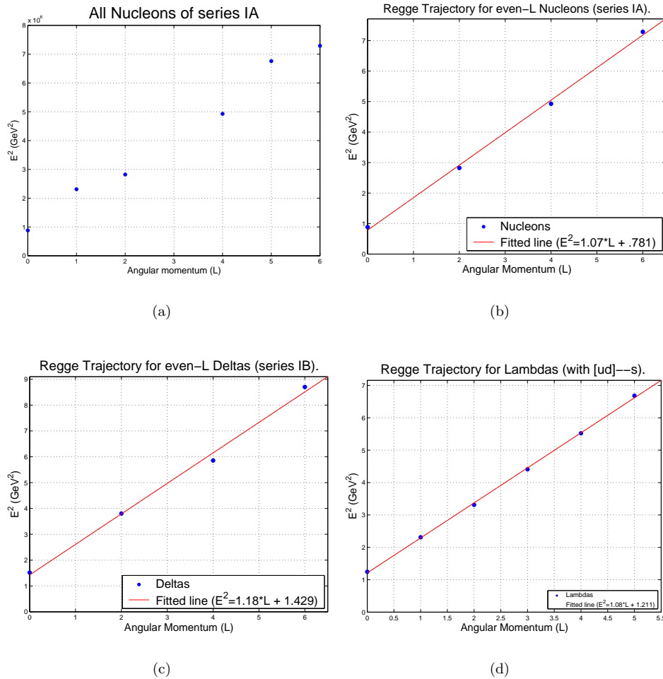
Figure 1. Various E^2 vs L plots. (a) is a plot of all Nucleons of series IA, showing “even-odd effect”. (b-d) are plots of the most prominent regge trajectories.
