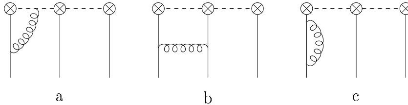
Figure 1. Examples of a “vertex” correction (a), “exchange” diagram (b) and self-energy insertion (c) contributing to the renormalization of three-quark operators in Feynman gauge. Path-ordered gauge factors are shown by the dashed lines. The set of all diagrams includes possible permutations.
